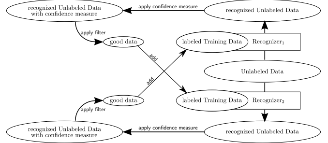
Figure 1. The approach to Co-Training investigated in this paper.
