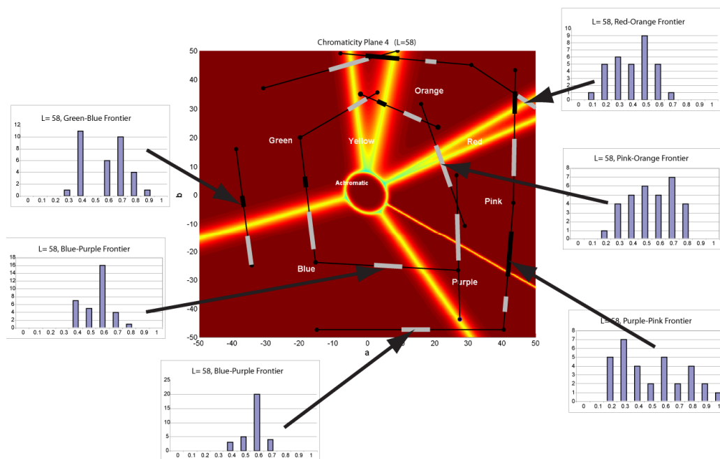
Figure 4: Experimental results for plane L=58 . The hotspots (pseudocolored radial lines in the central plot) represent the color name boundaries of the Benavente et al model 10 . Thresholds were measured for all observers along the solid lines on the chromaticity plane (central plot). The grey and black bars show the regions where the majority of the thresholds were measured. Some of the histograms showing the distribution of thresholds along the lines are shown as side-figures. The length of the bar is equal to the Standard Deviation of the measured thresholds.
