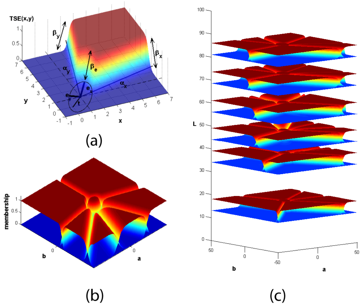
Figure 1: Fuzzy membership regions proposed by Benavente et al to segment the color space, based on a product of sigmoids and an elliptical centre. Panel (a) shows an individual TSE function, Panel (b) shows the combination of different TSEs to obtain the color space segmentation for a given value of L , and Panel (c) shows the six different levels of L as defined by the model.
