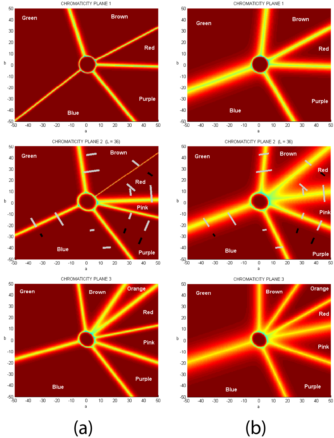
Figure 5: A new set of color name boundaries, adapted to fit our experimental results. (a) The initial boundaries for the model presented in Benavente et al 10 . (b) The readjusted model. The results of the experiment are superimposed on their corresponding plots.
