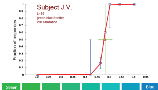
Figure 3: Exemplary result from a single experiment (for subject J.V.) involving the green-blue color-boundary (L=36, low saturation color pair). The solid line shows the psychometric function and the cross represents QUEST's mean threshold estimate.
