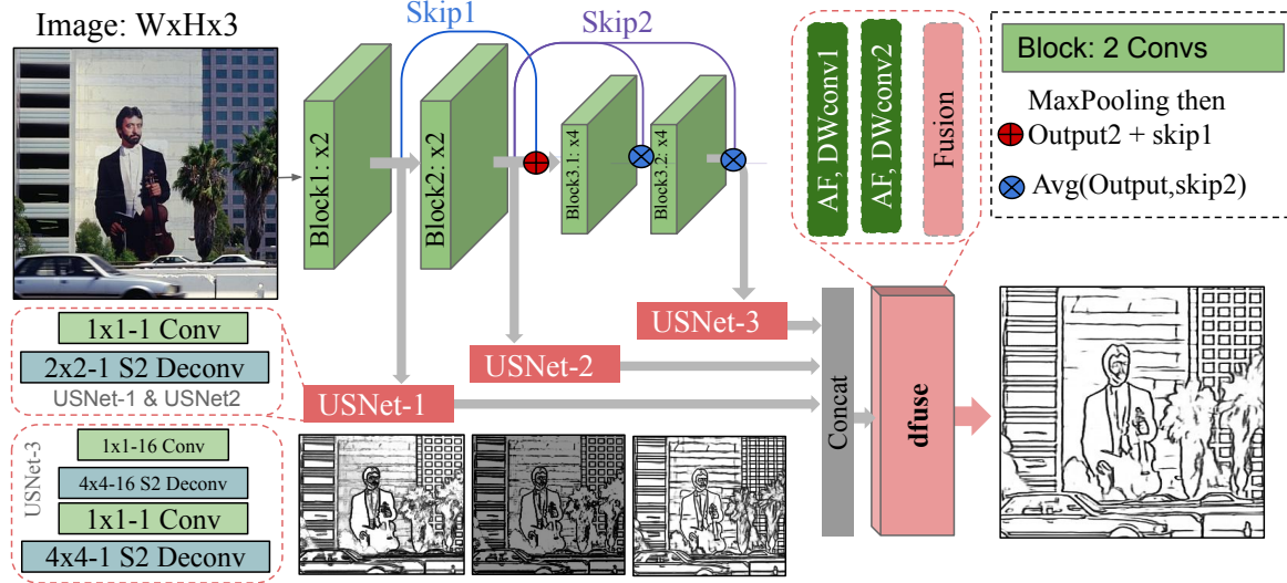
Figure 2: TEED architecture.
