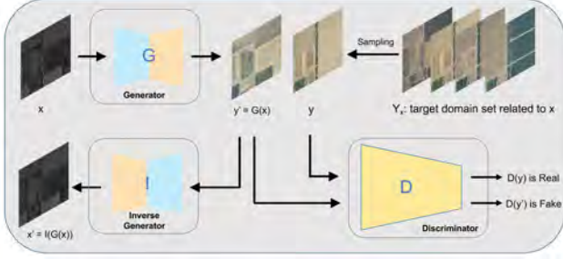
Figure 7. The MvAV-pix2pixHD method, designed for multi-view image translation tasks, features a generator (G) and discriminator (D) based on the coarse-to-fine and multi-scale principles of pix2pixHD, alongside an inverse generator (I) mirroring G’s structure but with independent training parameters. Using SAR2RGB as an example, SAR images are transformed into the RGB.
