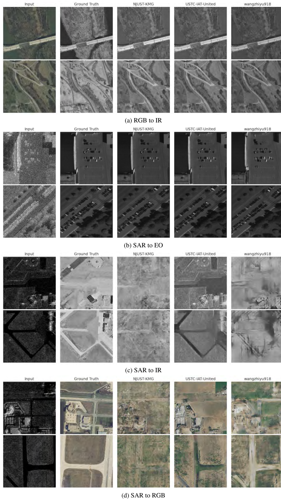
Figure 8. Comparison of the four translation task for the top three teams. The input and ground truth are given as well as the generated outputs for each of the to three teams.
