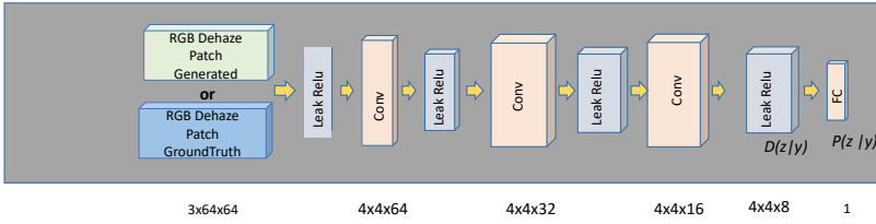
Fig. 1. Illustration of the proposed triplet cross-spectral dense CGAN architecture used for image dehazing.
