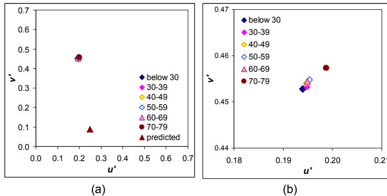
Figure 6 (a) Observer neutral grey settings and the predicted neutral grey for age 70-79; (b) Blown-up plot of observed settings
