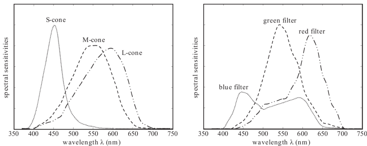
Figure 1. Spectral sensitivities of: (a) the three types of cones in a human eye, and (b) a typical digital camera. Images from [1].
